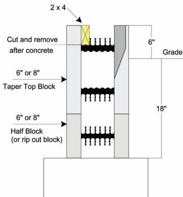
One and one half rows of Fox Blocks
