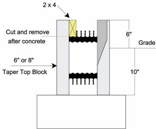
One row of Fox Blocks. Fox Blocks is designed to accept a 2 x 4 resting on top of the tie. Attach with screws through face of tie.
