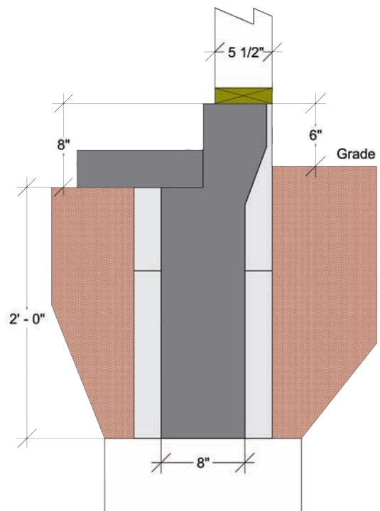
Using Curb Block allows you to lower slab to give a curb that does not require any finish. Taper is field cut into the top outside edge
